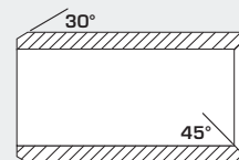
Form F WITH 45° countersink
