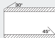
Form F WITH 45° countersink
