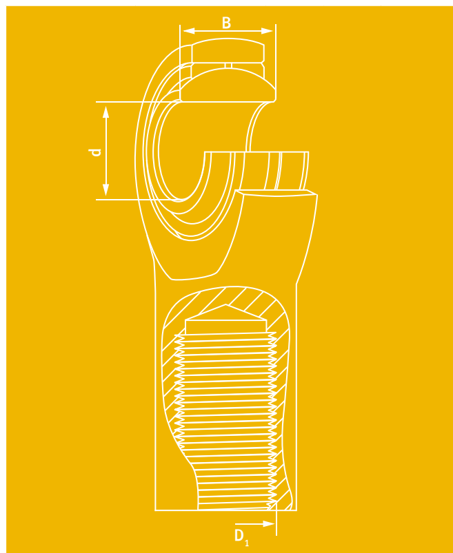
Rod end, steel / PTFE with inside thread
