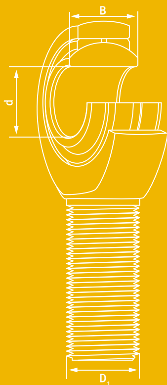
Rod end, rigid chrome / PTFE with outside thread
